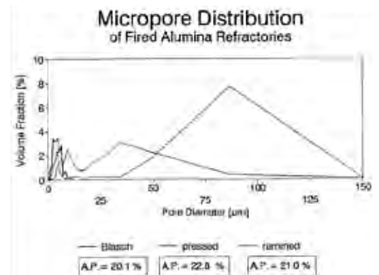
Figure 3. Micropore Distribution in Ceramics
