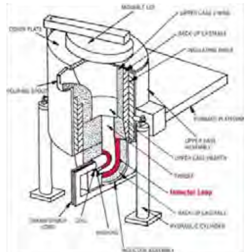
Figure 1. Channel Induction Furnace
